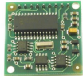
Compass module
